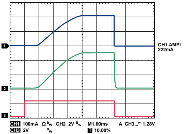
Figure 28. Typical Turn-On Delay Time with V_{IN} = 5.5V , I_{LOAD} = 220mA
