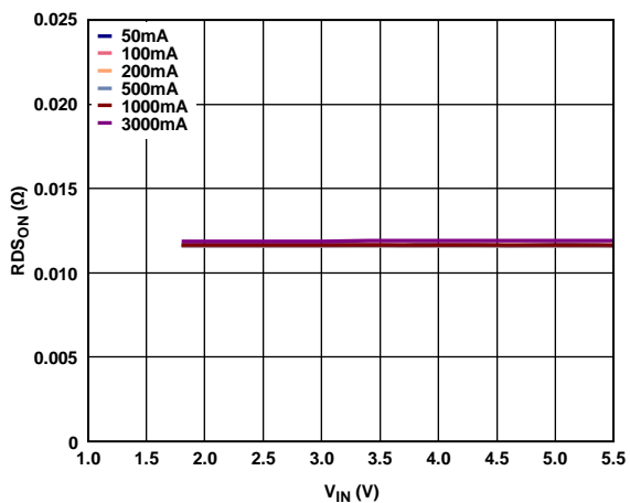
Figure 6. R_{DS(on)} vs. Input Voltage ( V_{IN} ), Different Load Currents
