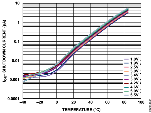
Figure 22. Output Shutdown Current vs. Temperature, V_{OUT} = 0\text{ V} , Different Input Voltages ( V_{IN} )
