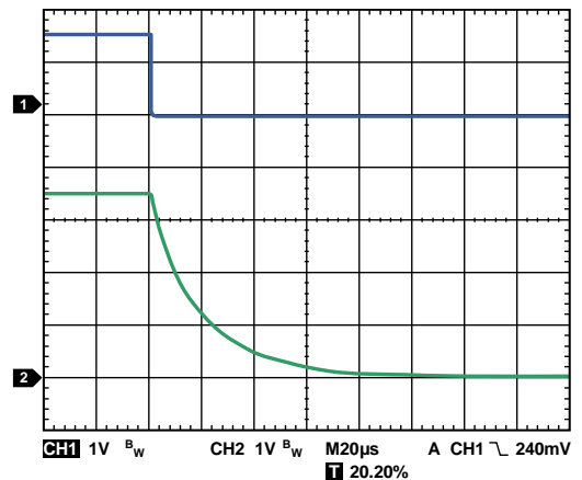
Figure 31. Typical Turn-Off Time
